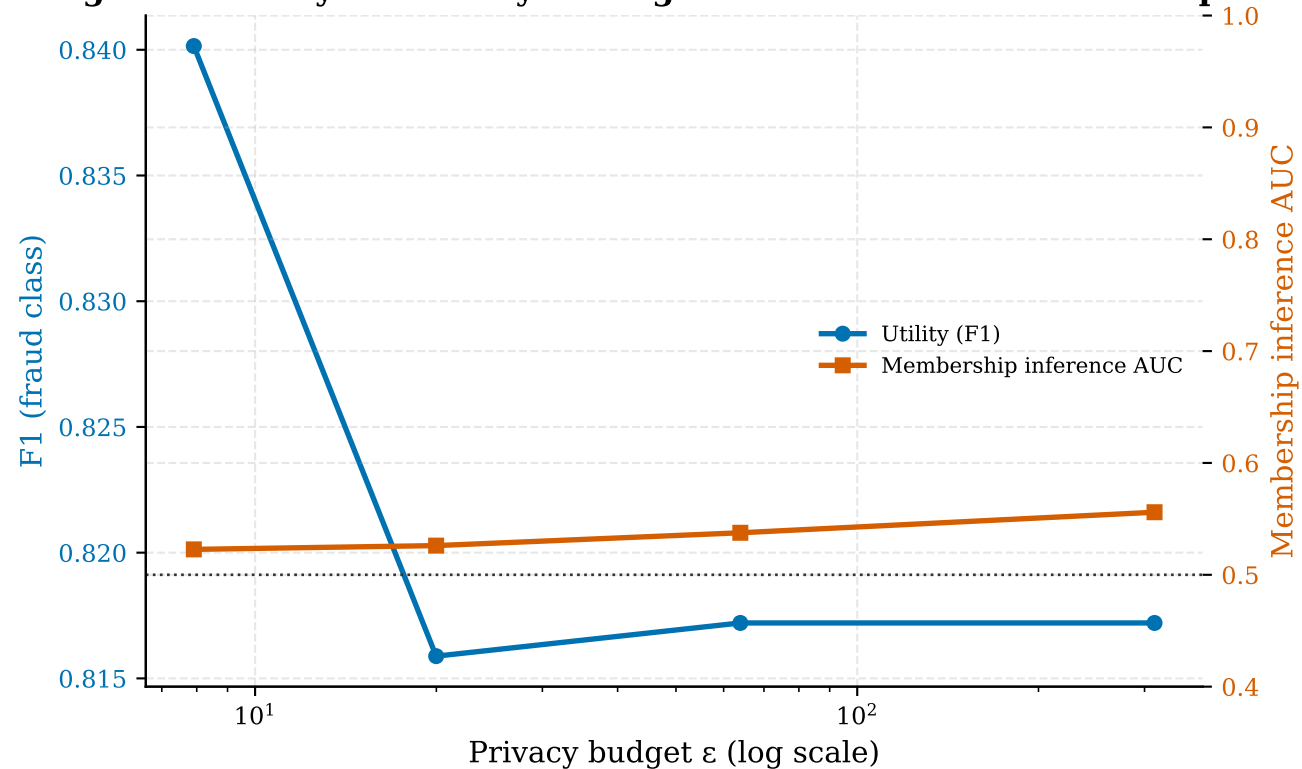
Figure 7. Utility vs. Privacy Leakage Across DP-SGD Noise Multipliers
